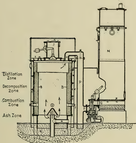
FIG. 94.—Fairbanks-Morse Suction Gas-Producer, Type 1.
